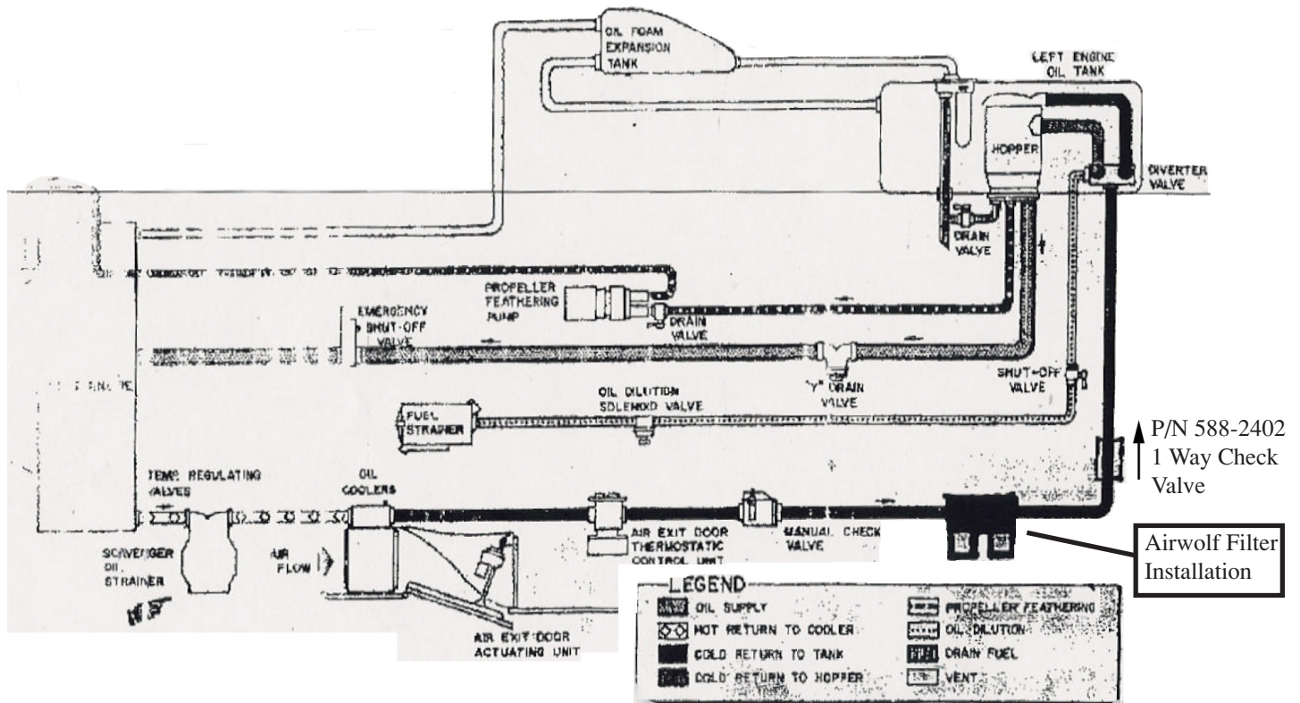
Figure 2-28. Engine Oil System Schematic
